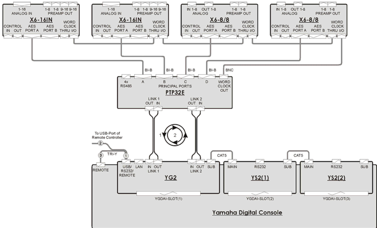
Fig. 5: Wiring of a system with PTP32(E), X6-converter units and a Yamaha console with YG2/YS2 cards. In order to control the X6-converter at the console the Yamaha Emulation Mode (YEM) must be activated in OPTOCORE CONTROL. Yamaha preamps connected to the PTP32(E) will use the fiber optical connection only for the bi-directional transfer of RS485 data and no special mode is activated.
