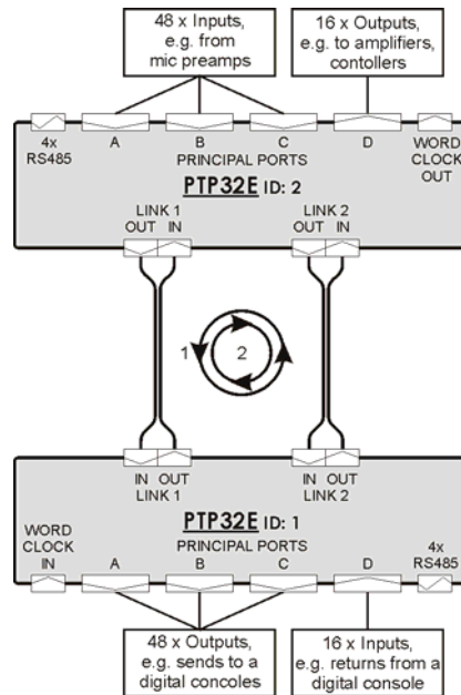
Fig. 1: Factory setting of a redundant Point-to-Point System
