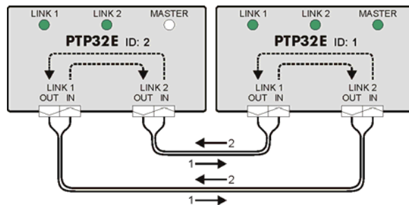
Fig. 3: Two PTP32E in a redundant Point-to-Point system
