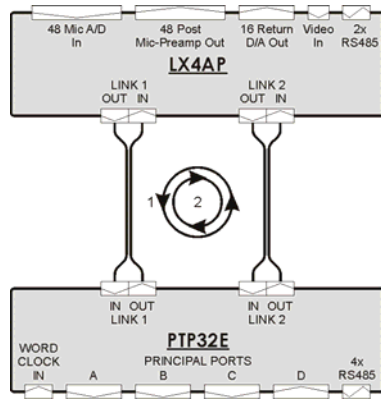
Fig. 4: Redundant system with one PTP32E and one LX4AP in a simple 48 send / 16 return configuration
