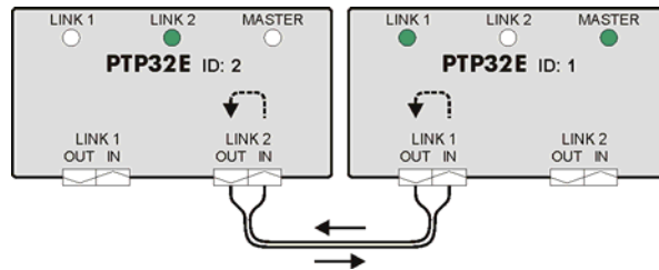
Fig. 2: Two PTP32E in a non-redundant Point-to-Point system
