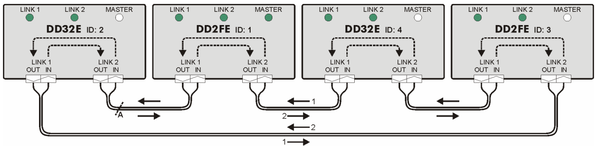
Fig. 2: Two DD2FE and two DD32E in a redundant network
