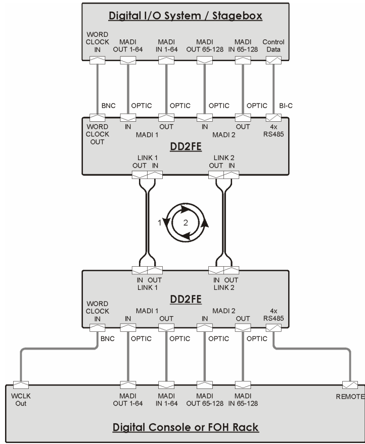
Fig. 3: Redundant network with two DD2FE in a 128 send / 128 return configuration
