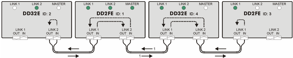
Fig. 1: Two DD2FE and two DD32E in a non-redundant network
