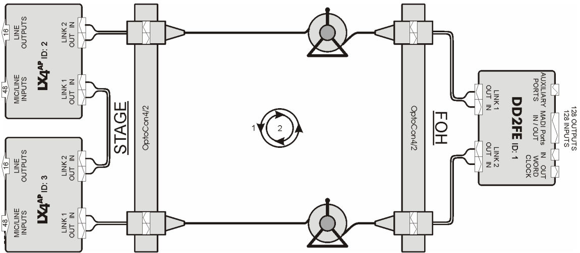
Fig. 4: Redundant network with one DD2FE, two LX4AP and OptoCon 4/2. 96 analog inputs and 32 analog outputs are available at the LX4AP's.
